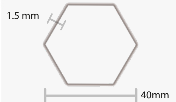
Hex Profile
